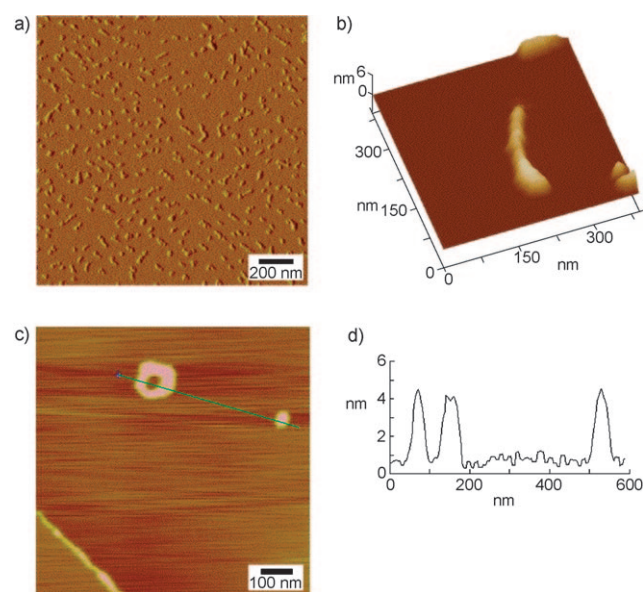
Figure 2. a)–c) AFM images of 2-apo-cyt b_{562} (H63C) assemblies on a HOPG substrate. d) The height profile along the green line in (c).
